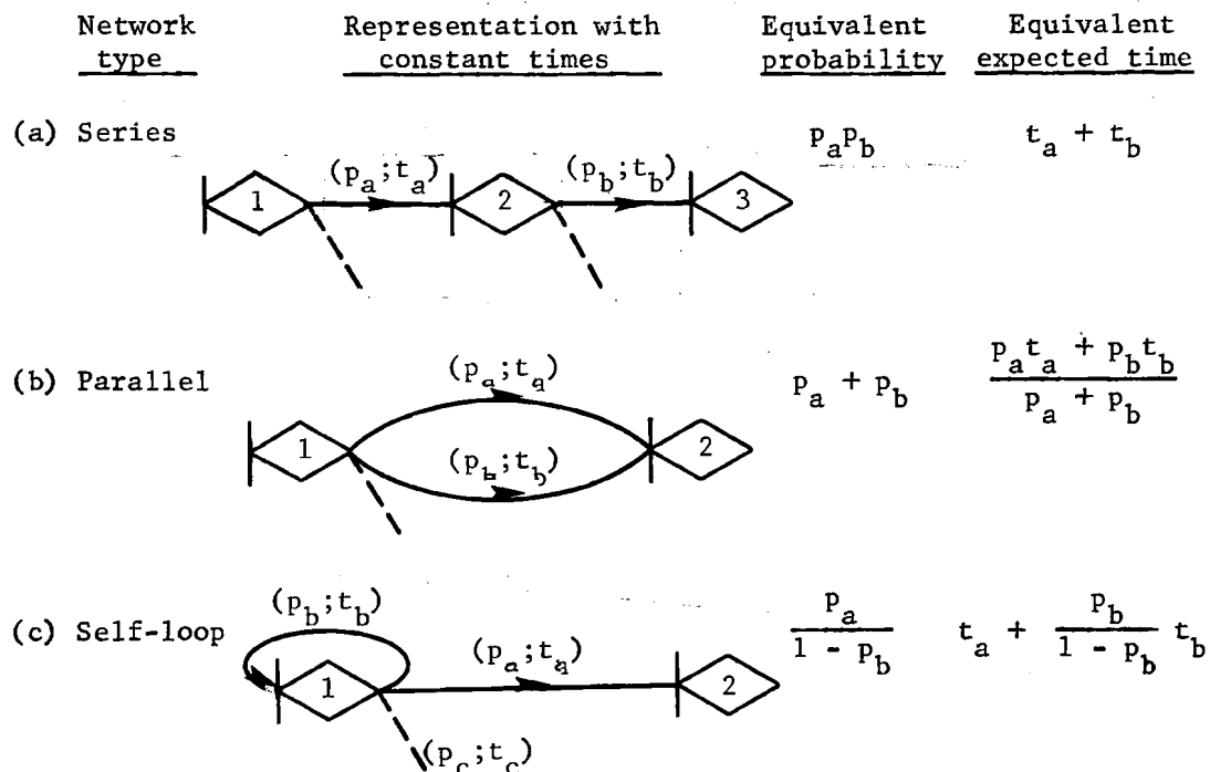
Fig. 1--Equivalence calculations of basic networks
